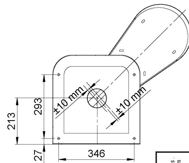
SECTION F-F
